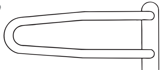
ANA-017-232 22 cm, 8 3/4" 20 x 65 mm ANA-017-233 22 cm, 8 3/4" 25 x 85 mm ANA-017-234 22 cm, 8 3/4" 25 x 120 mm ANA-017-235 22 cm, 8 3/4" 23 x 145 mm
