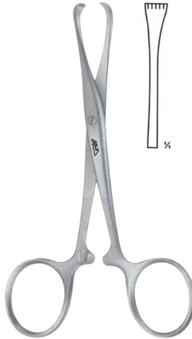
TUFFIER ANA-017-107 5 x 6 teeth, sharp 12.5 cm, 5"
