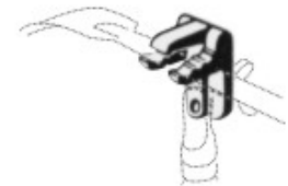
ANA-20-102 Support only, for brain spatulas with round shaft up to 5.5 mm diam. Fixing for flexible
